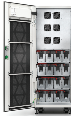
40 kVA Easy UPS 3S with internal batteries
